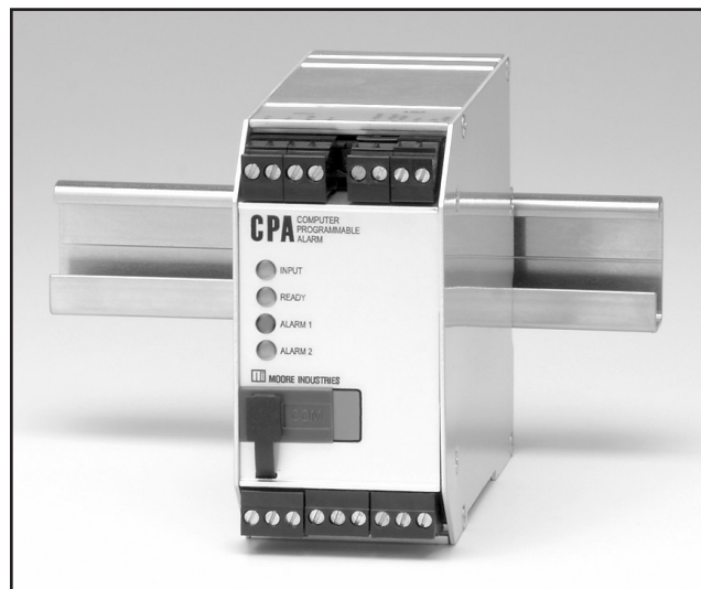
The CPA PC-Programmable Alarm features a metal, RFI resistant housing that snaps onto standard DIN-style rails.
