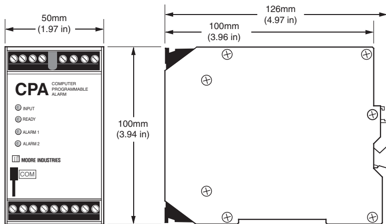
Figure 7. Installation Dimensions.
