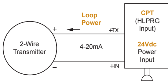
Figure 3. The CPT provides transmitter excitation to power a 2-wire transmitter.
