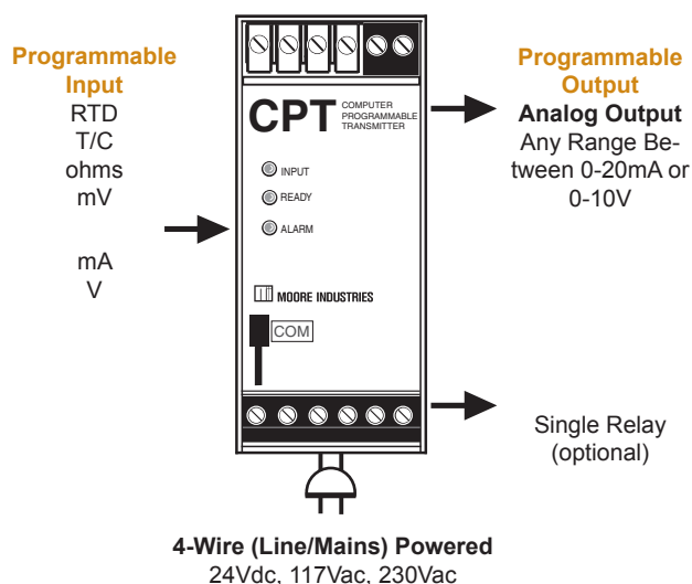
Figure 1. Available CPT models deliver versatile and programmable input and output choices.
