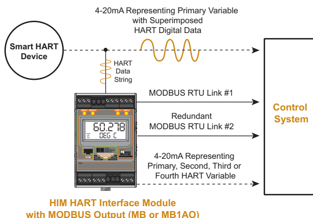
Figure 3. The HIM converts the HART digital protocol to MODBUS RTU (with MB or MB1AO output type).
