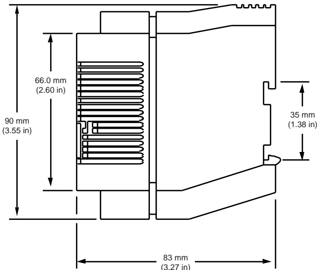
ALL MODELS (SIDE VIEW)
