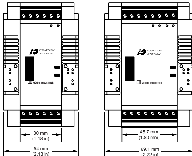
STANDARD MODEL (FRONT VIEW)
