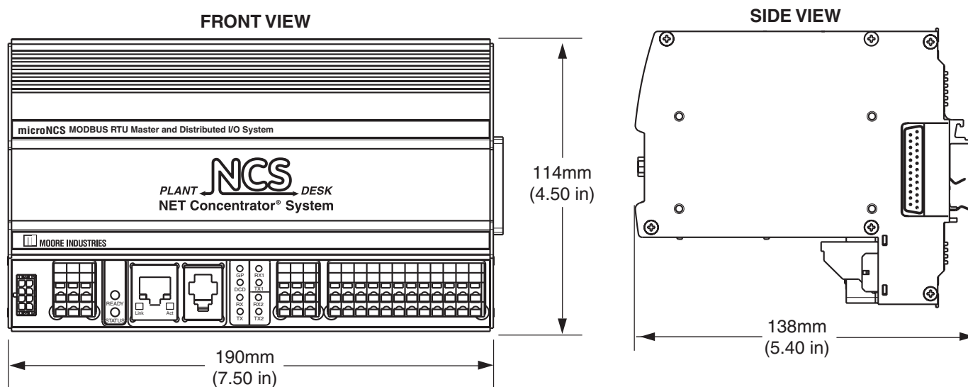
Figure 4. microNCS Dimensions (see the NCS NET Concentrator System data sheet for installation dimensions for expansion I/O).
