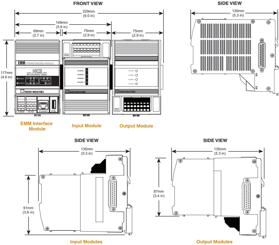
Figure 9. Installation Dimensions.
