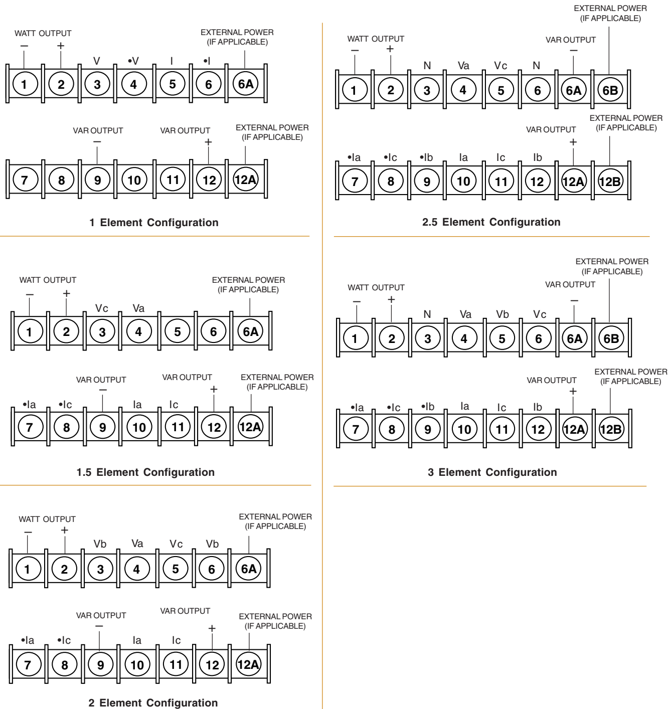
Figure 4. PWV Terminal Designations
