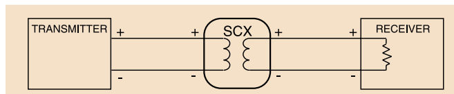
Figure 1. The SCX provides complete isolation between a transmitted signal source and a receiving device.
