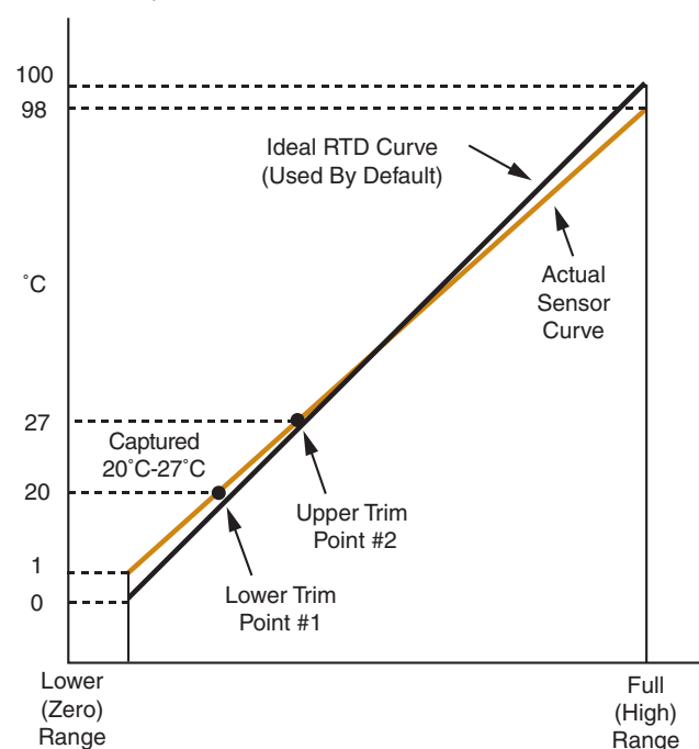
Figure 9. The SPA 2 can be set to measure the segment most critical to the process.
