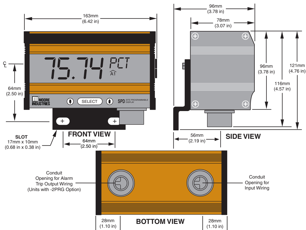
Figure 2. Installation Dimensions
