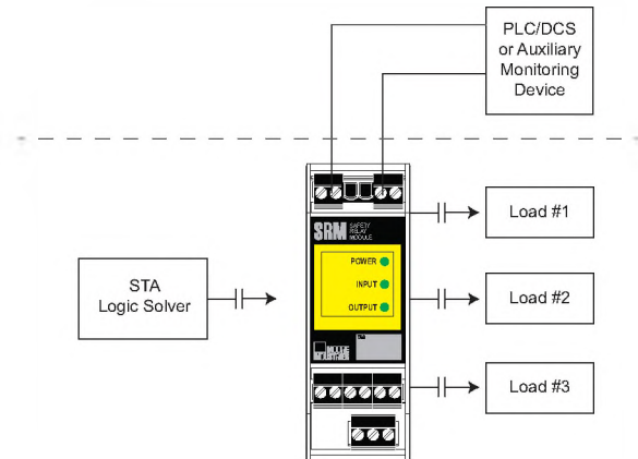
Figure 3. The Monitor and Input contacts of the SRM may be connected to a PLC, DCS or other monitoring device for diagnostic purposes.
