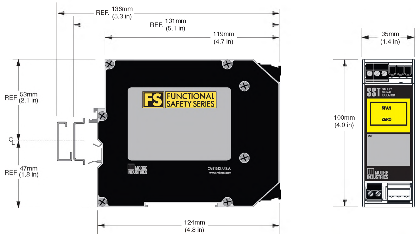
Figure 10. Dimensions of the SST Isolator in its aluminum DIN-style housing
