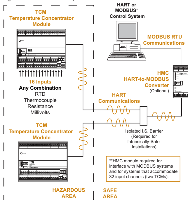
Figure 1. One or two* 16-channel temperature concentrator modules (TCM) can be used on the same network to allow up to 32 signals to be economically transmitted back to the control room.
