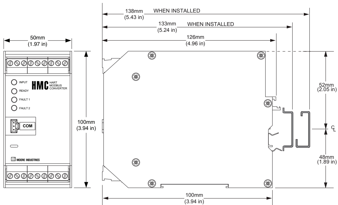
Figure 7. HMC HART-to-MODBUS Converter Dimensions.
