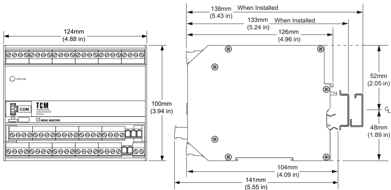
Figure 6. TCM Temperature Concentrator Module Dimensions.
