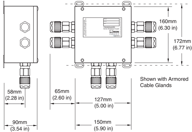
Figure 8. Stainless Steel 316 with E-Z Vertically Removable Lid and Bottom Entry Cable Gland Plate Installation Dimensions for 8-Spur (TG248), 10-Spur (TG24X), 12-Spur (TG2W) and 20-Spur (TG24Y) Models.
