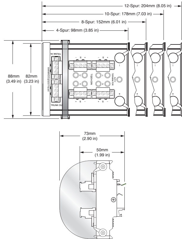
Figure 5. Standard Aluminum Enclosure Installation Dimensions for 4-Spur (TG25/64), 8-Spur (TG25/68), 10-Spur (TG25/6X) and 12-Spur (TG25/6W) Models.
