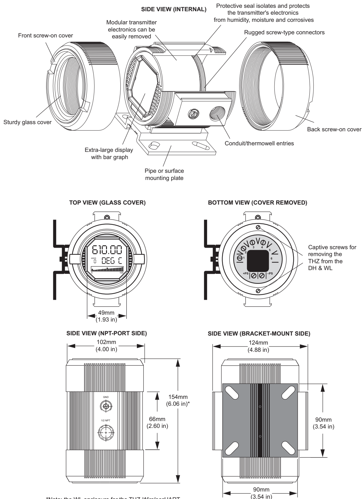
Figure 7. Dimensions for the THZ in DH and WL dual compartment enclosures.
