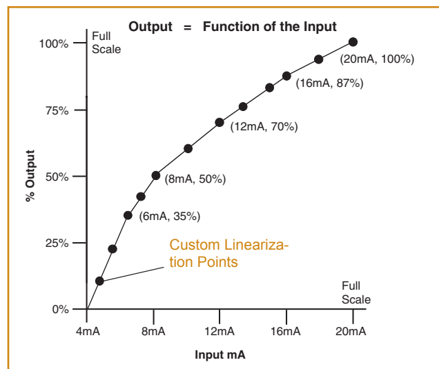
Figure 6. Custom linearization points can be selected and saved in the TMZ's memory to compensate for non-linear input signals.
