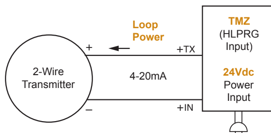
Figure 5. The TMZ provides transmitter excitation to power a 2-wire transmitter.
